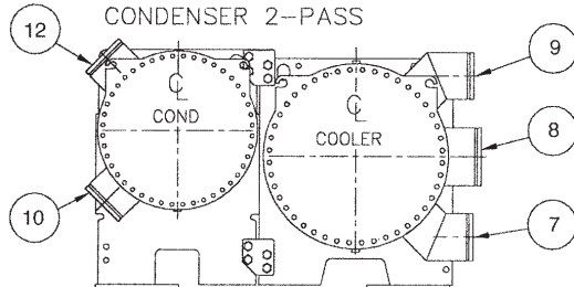
DISCHARGE END
